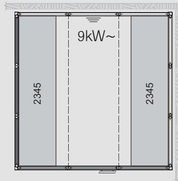
PANACEA STEAM 2525 SIZE: 2525 x 2525
